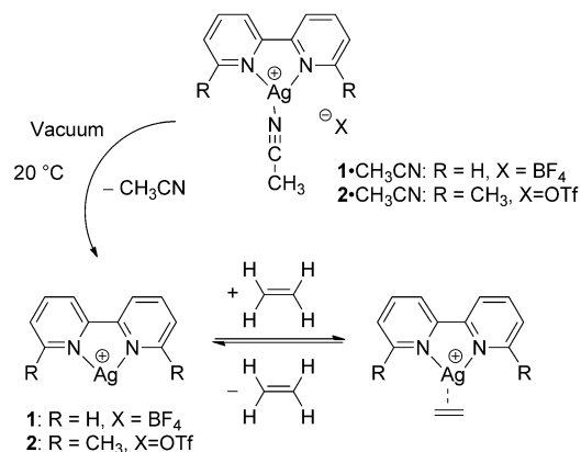
Scheme 1. The mild activation of 1 · \text{CH}_3\text{CN} and 2 · \text{CH}_3\text{CN} to form the solid-state materials 1 and 2 , which exhibit reversible and selective ethene versus ethane binding. Tf = trifluoromethanesulfonyl.
